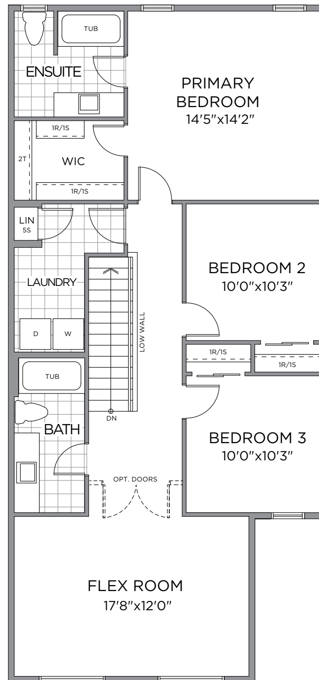
SECOND FLOOR
