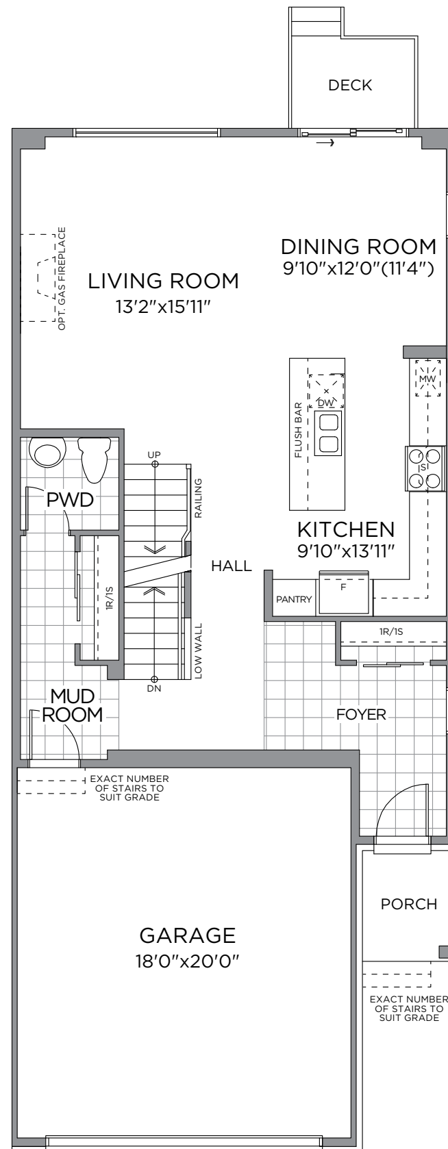
GROUND FLOOR
