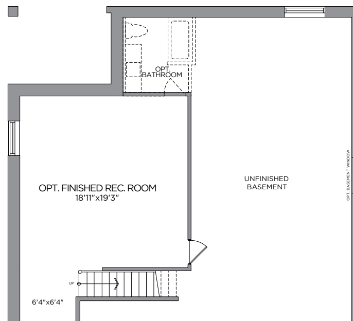
OPT. FINISHED BASEMENT REC. ROOM 477 SQ. FT.
