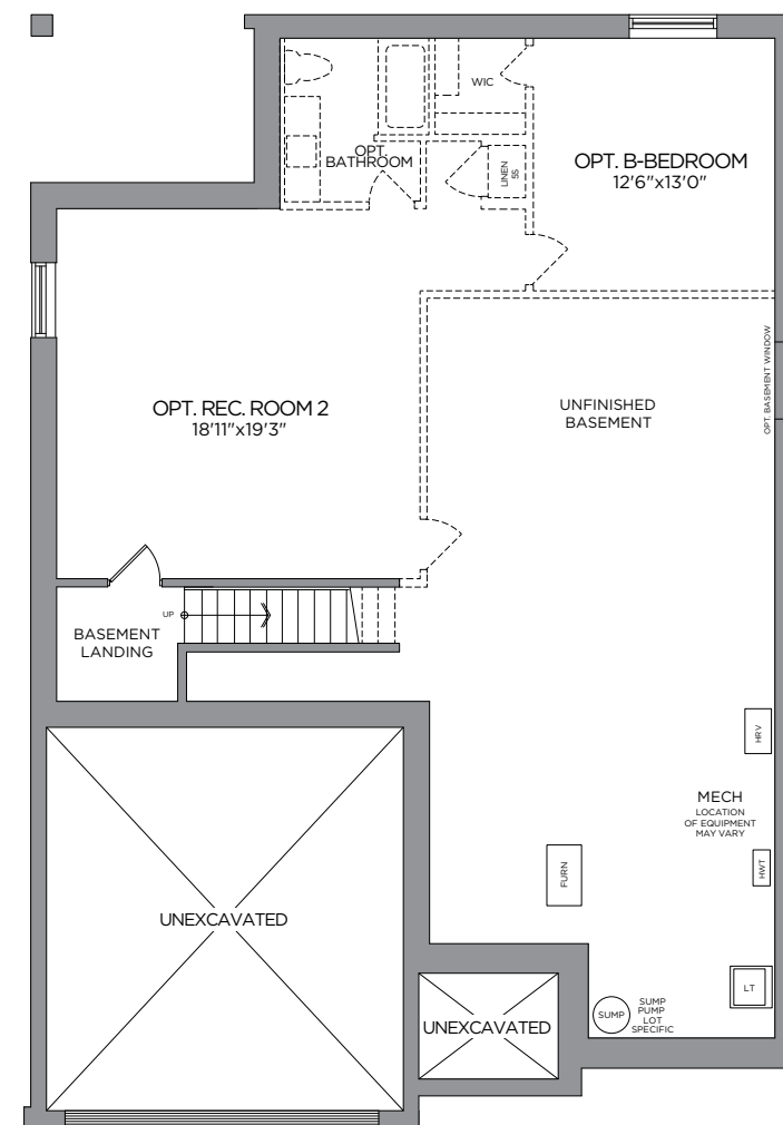
STANDARD BASEMENT PLAN OPT. FINISHED BASEMENT 844 SQ. FT.
