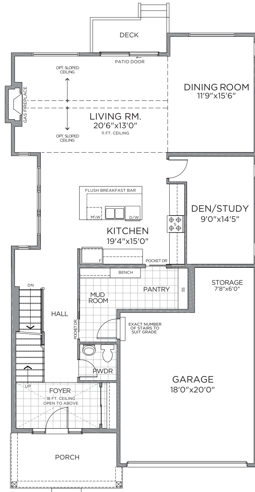
GROUND FLOOR
