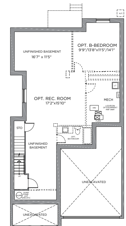
STANDARD BASEMENT PLAN OPT. FINISHED BASEMENT PLAN 1074 SQ. FT.
