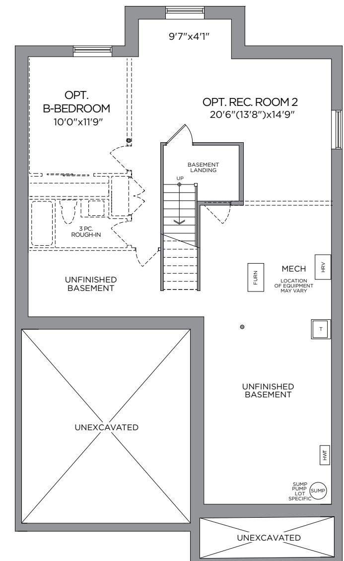
STANDARD BASEMENT PLAN OPT. FINISHED BASEMENT PLAN 662 SQ. FT.
