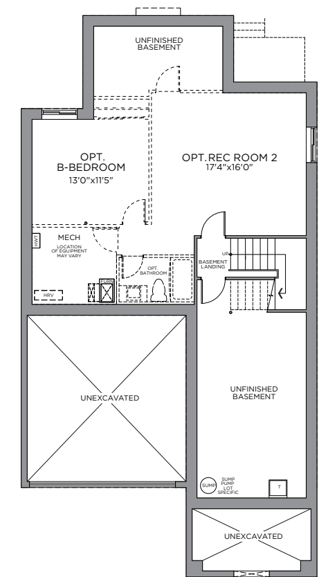
STANDARD BASEMENT PLAN OPT. FINISHED BASEMENT PLAN 623 SQ. FT.
