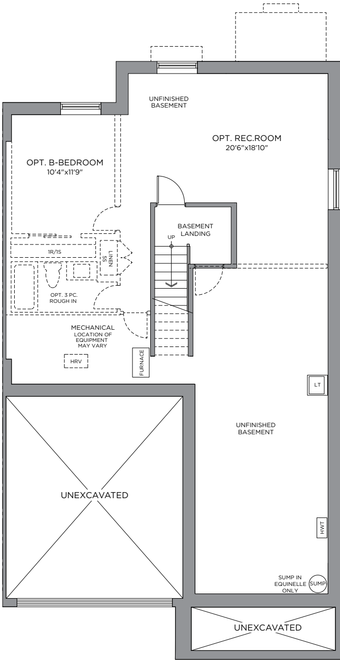
STANDARD BASEMENT PLAN OPTIONAL FINISHED BASEMENT PLAN 705 SQ. FT.
