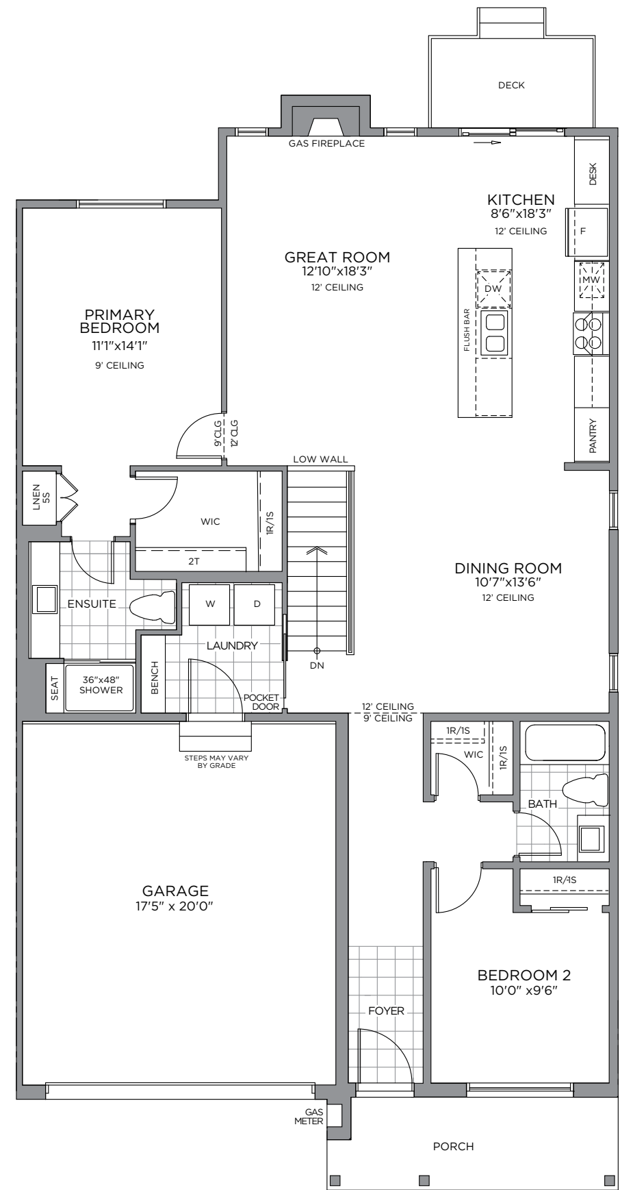
GROUND FLOOR
