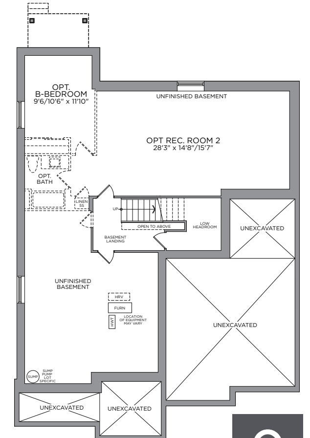
STANDARD BASEMENT PLAN OPT. FINISHED BASEMENT 852 SQ. FT.
