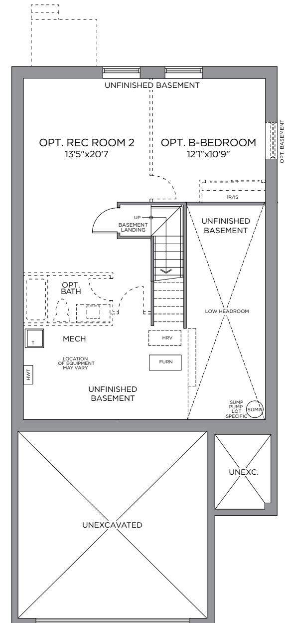
STANDARD BASEMENT PLAN OPT. FINISHED BASEMENT PLAN 553 SQ. FT.
