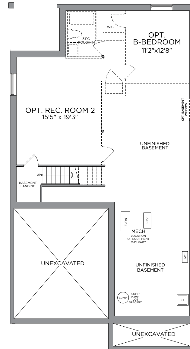
STANDARD BASEMENT PLAN OPT. FINISHED BASEMENT PLAN 709 SQ. FT.
