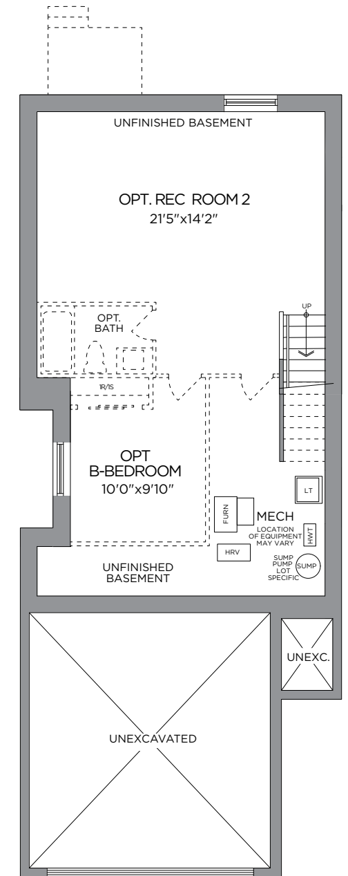
STANDARD BASEMENT PLAN OPT. FINISHED BASEMENT PLAN 636 SQ. FT.
