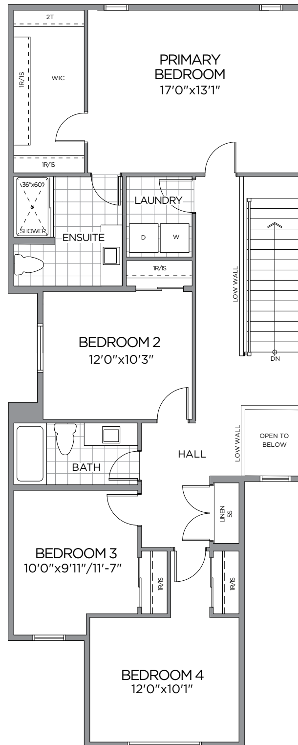
SECOND FLOOR
