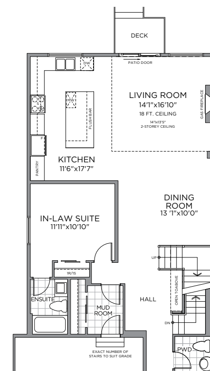
OPT. GROUND FLOOR W/ IN-LAW SUITE ELEV. B
