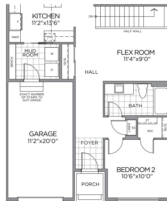
OPT. GROUND FLOOR PLAN
